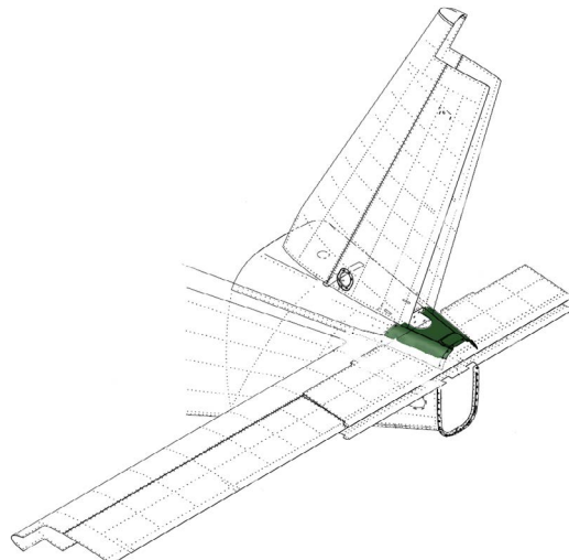
Figure 1: Rudder Closeout Fairing
